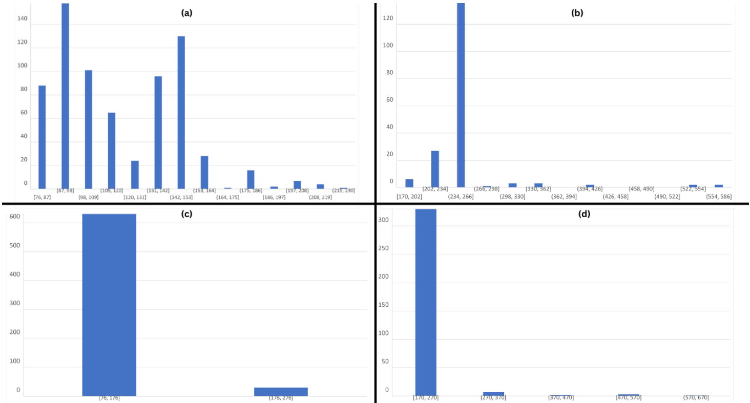
Figure 10: Each plot shows how the same type of data can look different depending on its natural spread and the bin width used. (a) Dataset with large spread and small bin width(17). (b) Dataset with small spread and small bin width(17). (c) Dataset with large spread and large bin width(100). (d) Dataset with small spread and large bin width(100).
