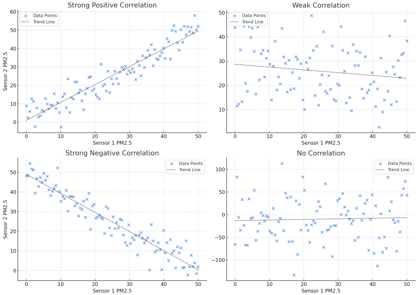
Figure 11: The scatter plots show four types of relationships: (a) strong positive correlation, (b) weak negative correlation, (c) strong negative correlation, and (d) no correlation. The black dotted line represents the best-fit trend line for each case. Strong correlations (positive or negative) indicate that the datasets change together in a predictable manner, while weak or no correlation suggests random, unrelated variations.
