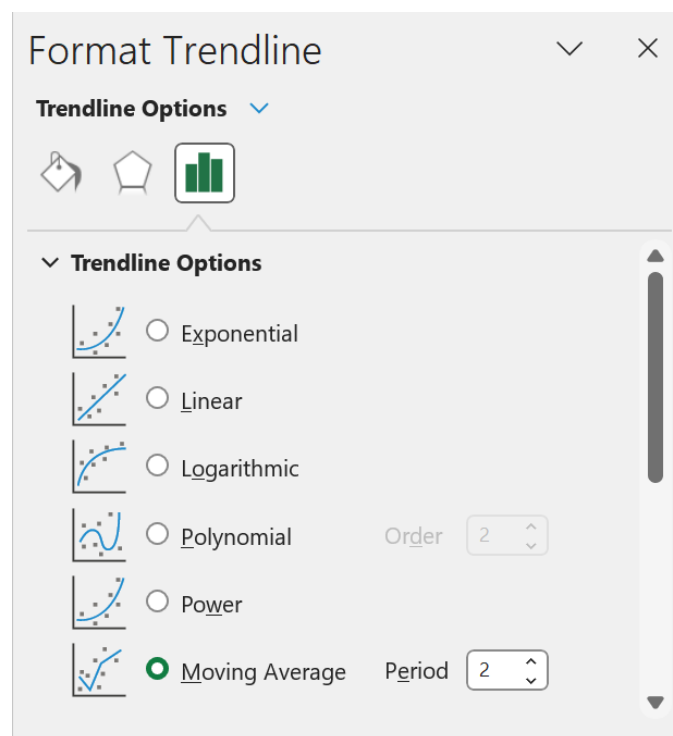
Figure 9: Adjusting period length of rolling average using trendline options in Excel.
